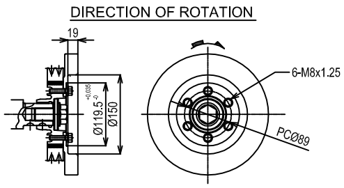
DETAIL OF PULLEY VIEWED FROM A
