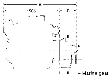
With YX120 gearbox / Left side view
