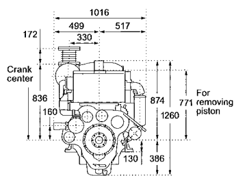
Engine only / Front view
