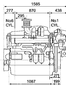
With YX120 gearbox / Left side view
